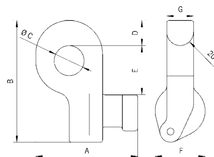
Model TCU
